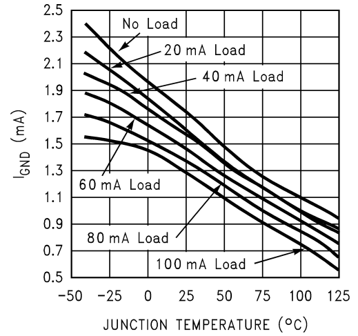
Ground Pin Current vs Junction Temperature
